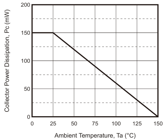
Fig.6 - P_C - T_a
