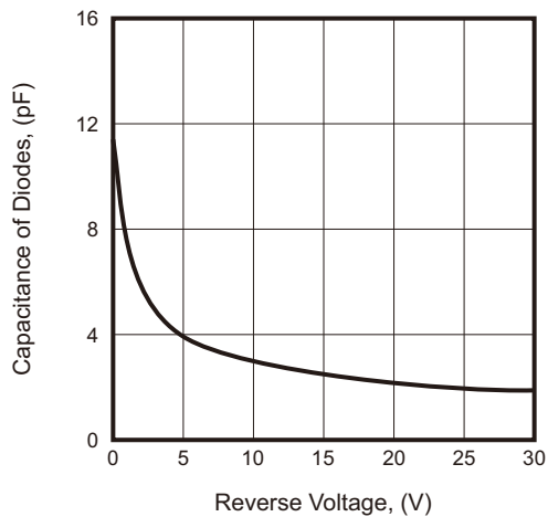
Fig.3 - Capacitance of Diodes
