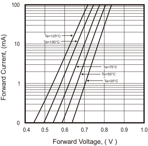
Fig.4 - Forward Characteristic
