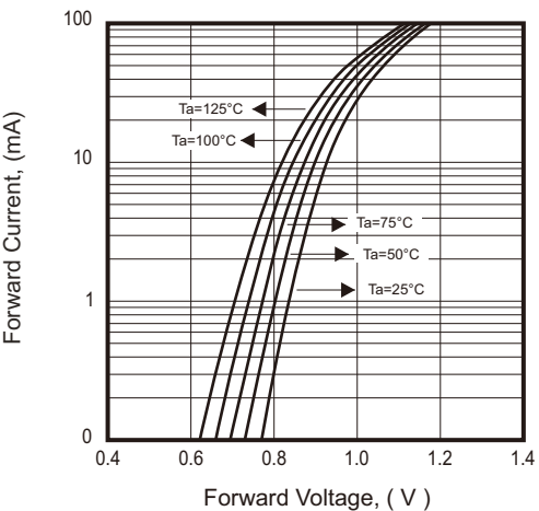
Fig.4 - Forward Characteristic
