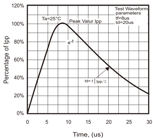
Fig.1 - 8/20us Peak Pulse Current Waveform Acc. IEC 61000-4-5
