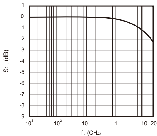
Fig.5 - Insertion Loss, Typical Values
