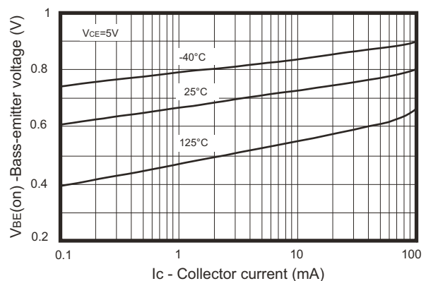
Fig.4 Base-Emitter ON voltage V.S. Collector current
