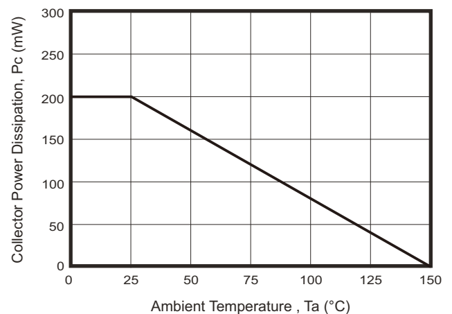
Fig.8 - P_c - T_a
