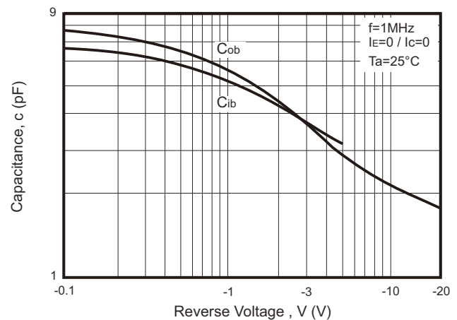
Fig. 6 - C_{ob}/C_{ib} - V_{CB}/V_{EB}
