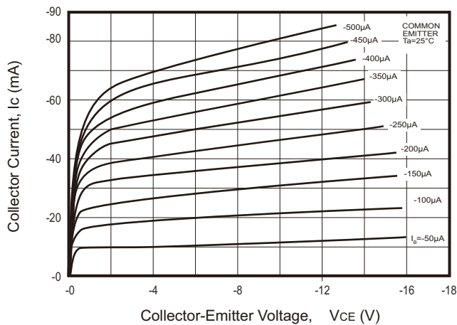
Fig.1 - Static Characteristic
