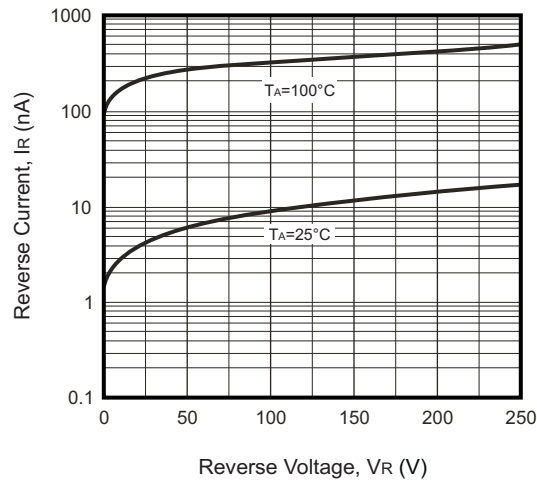
Fig.2 - Reverse Characteristic
