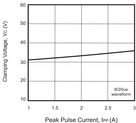
Fig.3 - Typical Clamping Voltage Vs. Peak Pulse Current
