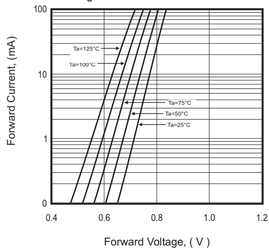
Fig.4 - Forward Characteristic
