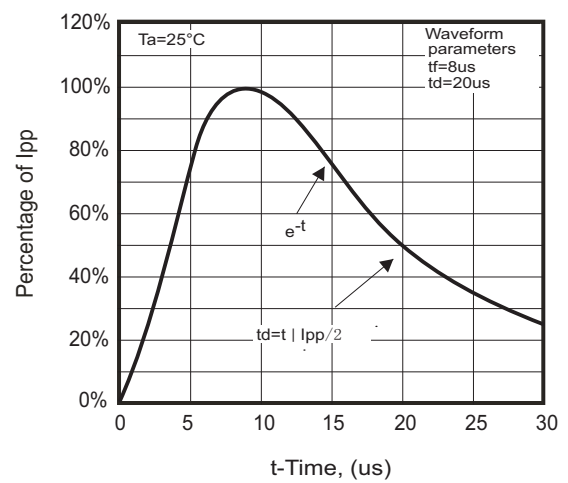
Fig.4- Pulse Waveform
