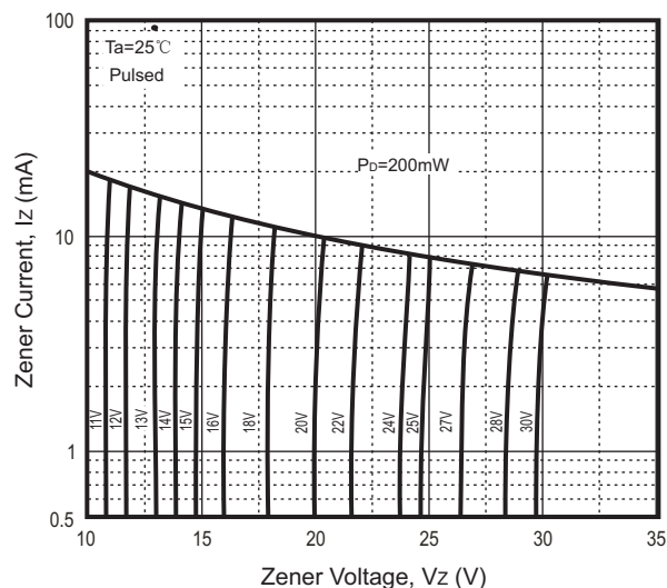
Fig.2 - Zener Characteristics (11V to 30V)
