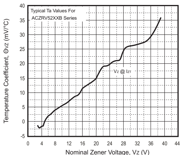
Fig.3 - Temperature Coefficients
