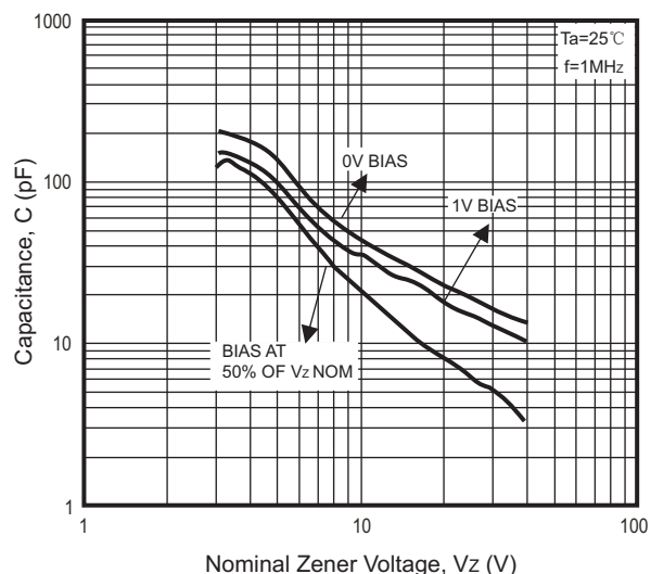
Fig.4 - Typical Capacitance
