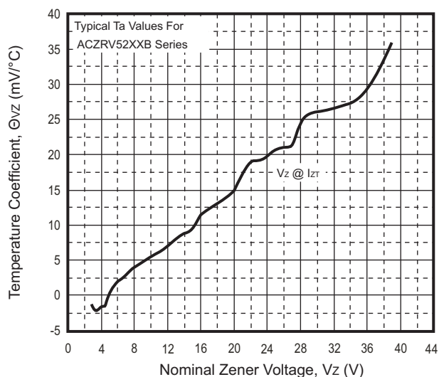
Fig.3 - Temperature Coefficients
