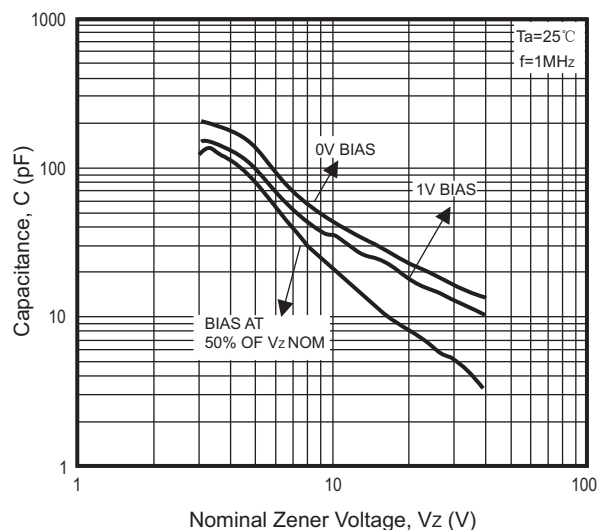
Fig.4 - Typical Capacitance
