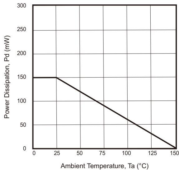
Fig.2 - Derating Curve
