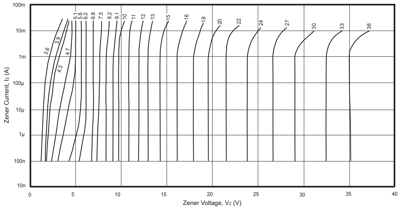
Fig.1 - Zener Voltage Characteristics
