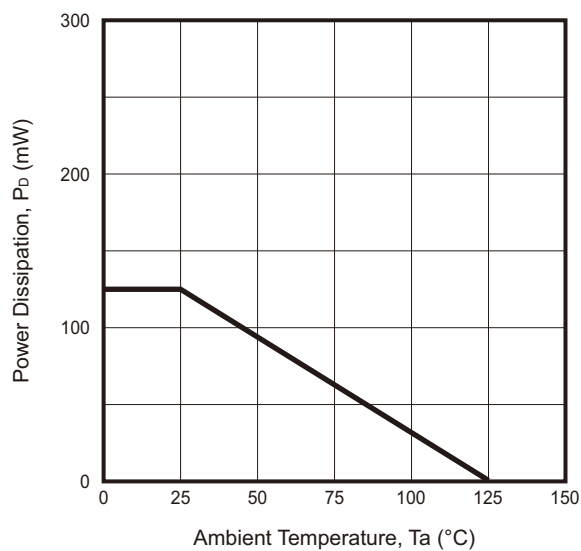
Fig.2 - Derating Curve
