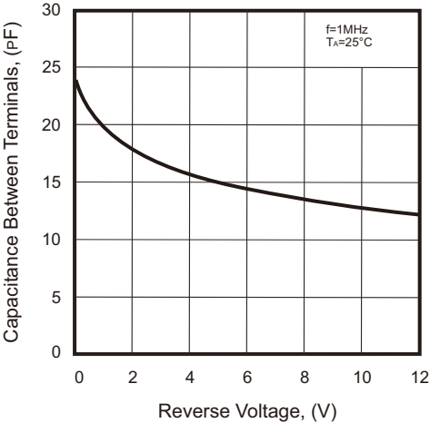
Fig.4 - Typical Capacitance Between Terminals Characteristics
