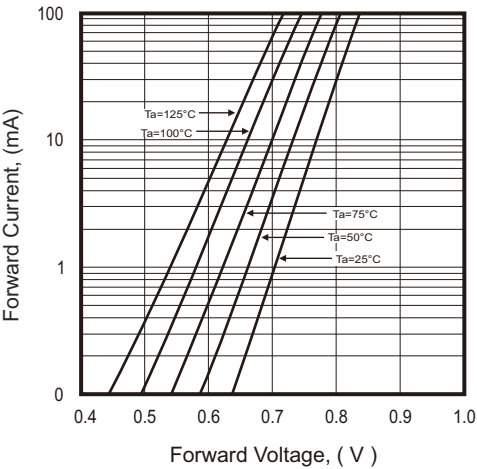
Fig.4 - Forward Characteristic
