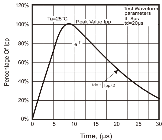
Fig.1 - 8/20μs Peak Pulse Current Wave Form Acc. IEC61000-4-5
