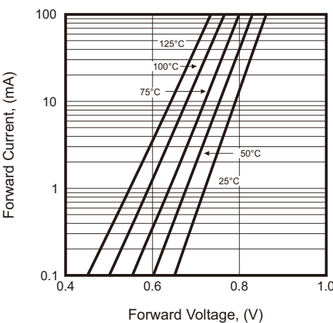
Fig.5 - Forward Characteristic
