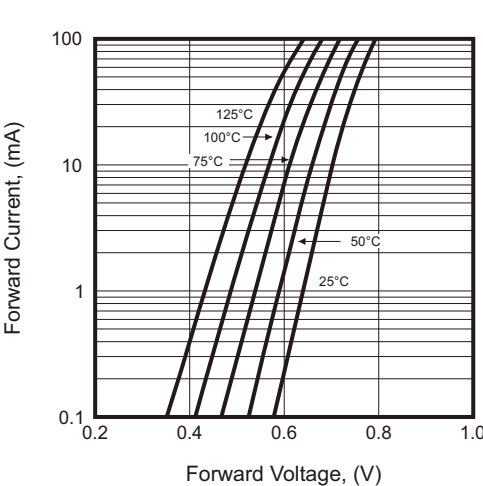
Fig.5 - Forward Characteristic
