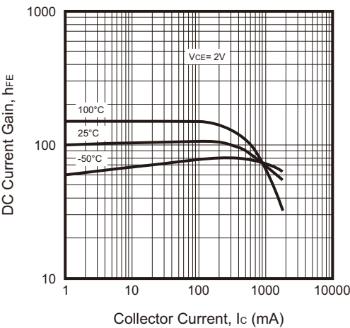
Fig.1 - h_{FE} — I_C
