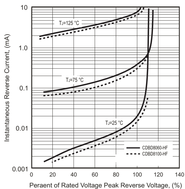
FIG.4-Typical Reverse Characteristics
