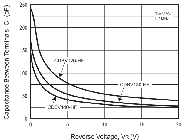
Fig.2- Capacitance Characteristics
