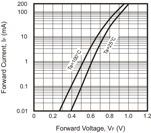
Fig.1 - Forward Characteristics
