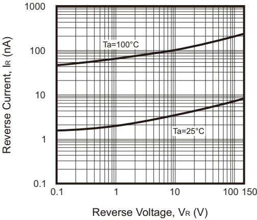
Fig.2 - Reverse Characteristics
