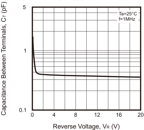
Fig.3 - Capacitance Characteristics Per Diode
