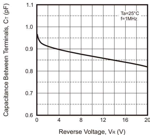
Fig.3 - Capacitance Characteristics
