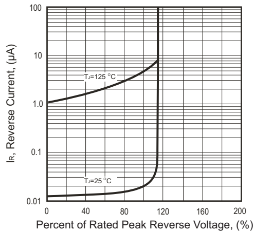
Fig.1- Reverse Characteristics
