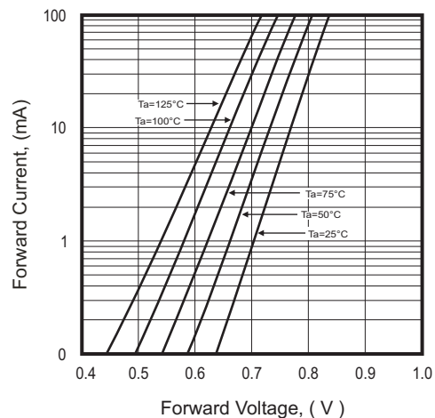
Fig.4 - Forward Characteristic
