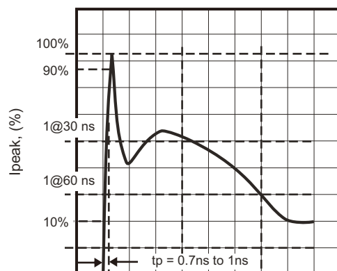
Fig.5 - IEC61000-4-2 Waveform
