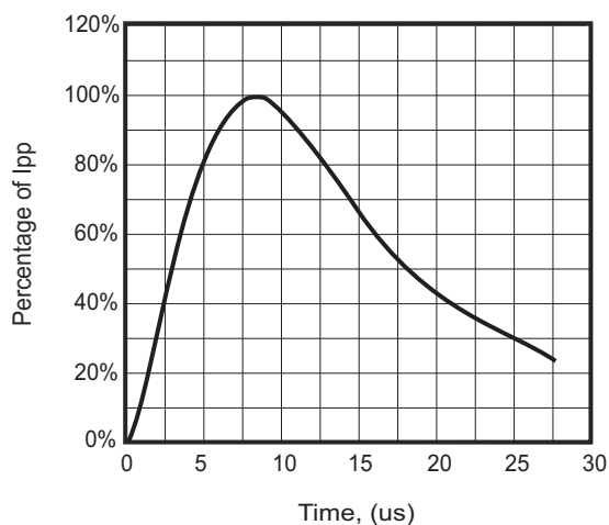
Fig. 5 - Pulse Waveform
