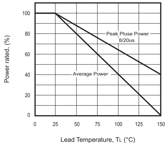
Fig.2 - Power Derating
