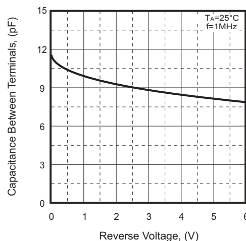
Fig.2 - Capacitance Characteristics
