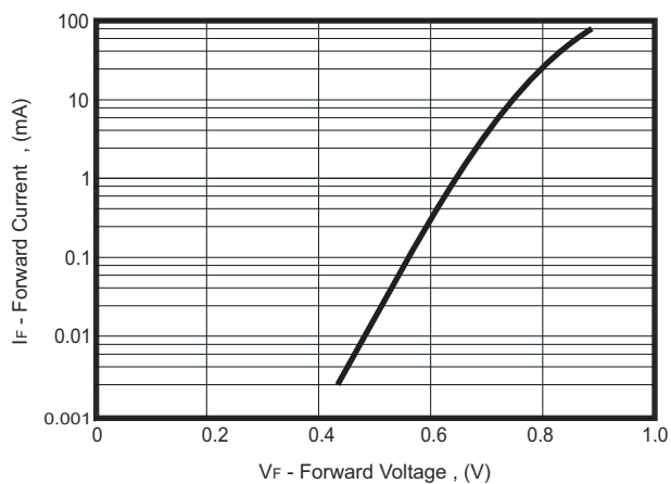
Fig.7 Forward Current Forward Voltage
