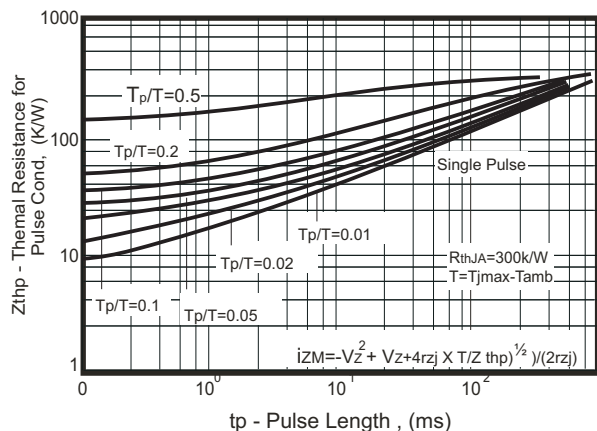
Fig.11 Thermal Response
