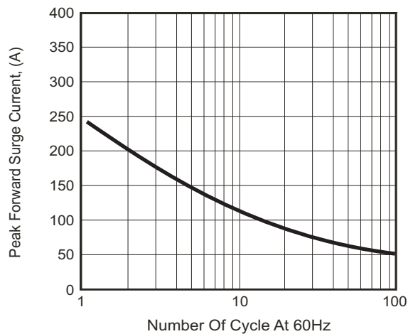
Fig.2 - Max. Forward Surge Current
