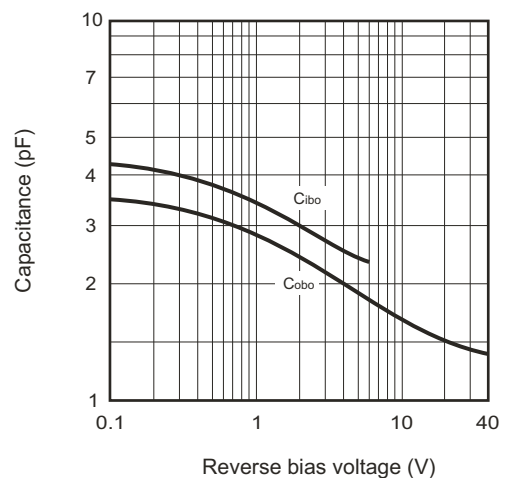
Fig.6 - Capacitance
