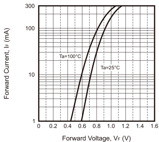
Fig.1 - Forward Characteristics
