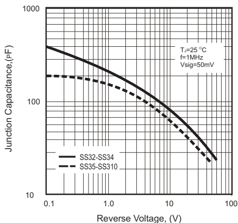
Fig.1 Typical Junction Capacitance
