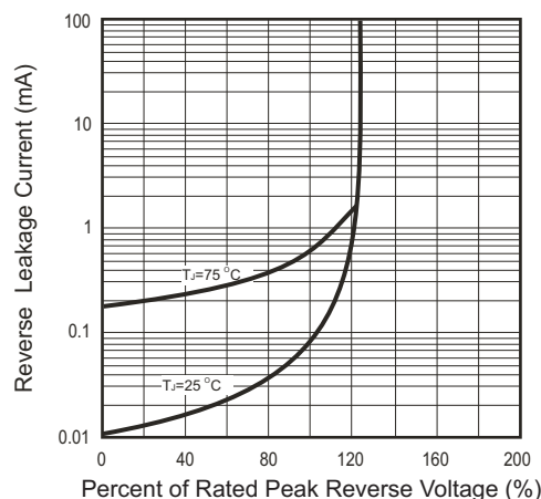
Fig.5 - Reverse Characteristics
