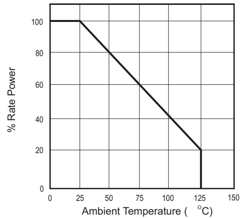
Fig.2 Power Derating
