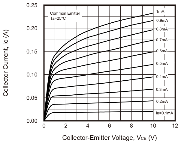
Fig.1 - Static Characteristic
