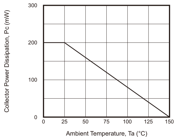
Fig.8 - P_c — T_a
