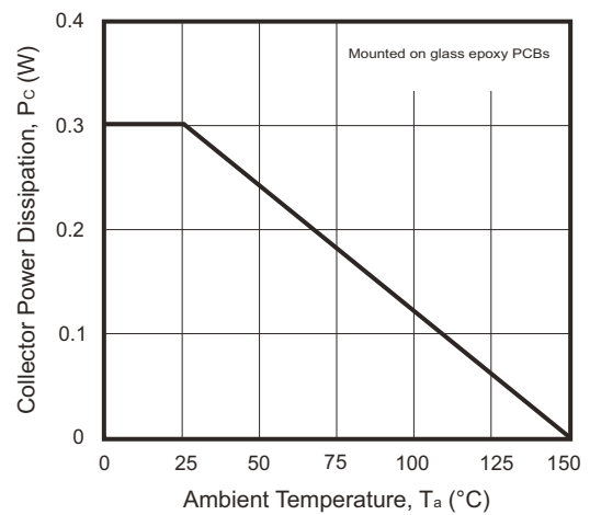
Fig.8 - P_c — T_a
