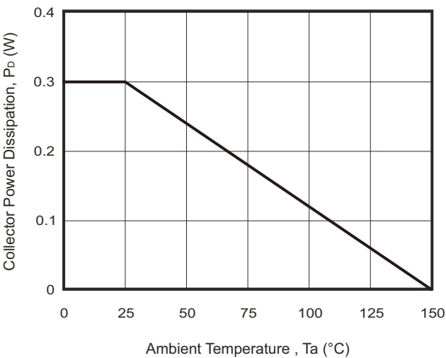
Fig.8 - P_C — T_a
