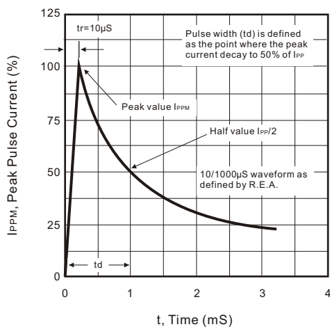
Fig.3 Pulse Waveform
