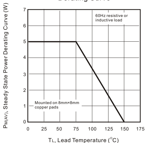
Fig.5 Steady State Power Derating Curve
