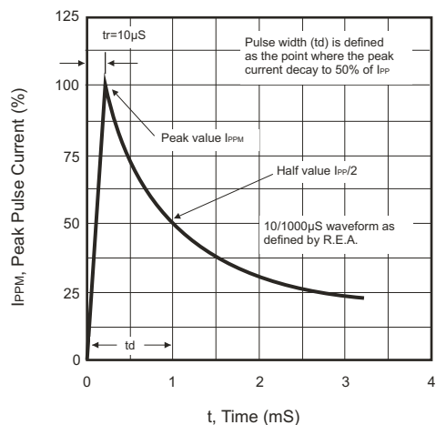
Fig.3 Pulse Waveform
