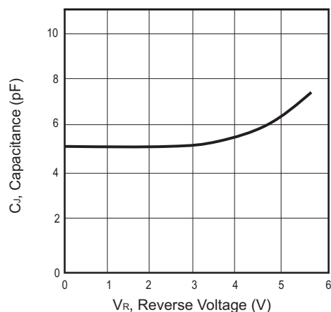
Fig.6 Capacitance vs. Reverse Voltage
