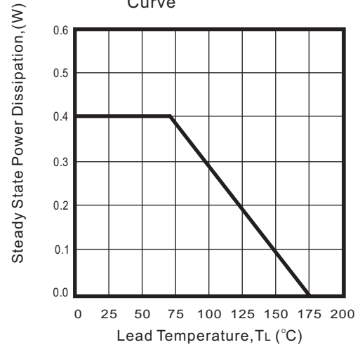
Fig.2 -Steady State Power Derating Curve
