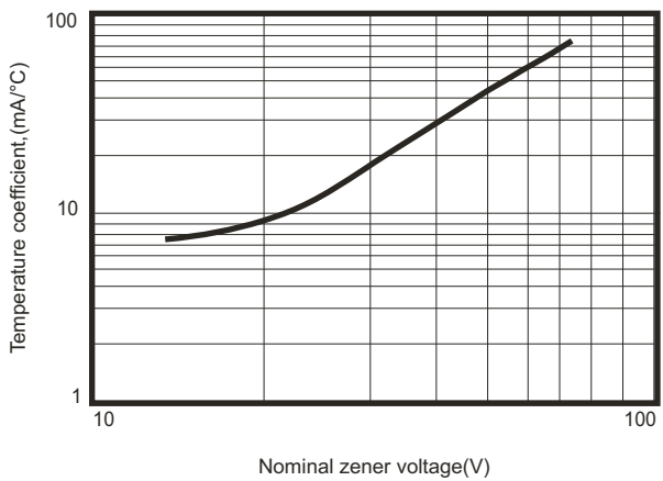
Fig.3 Temperature coefficients
