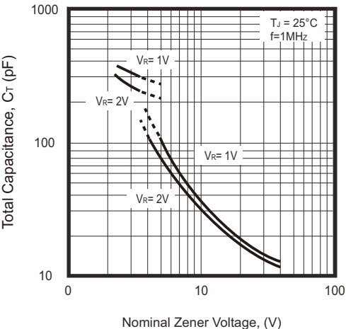
Fig.5 - Total Capacitance vs Nominal Zener Voltage
