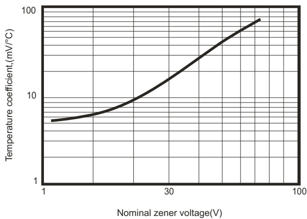
Fig.3 Temperature coefficients
