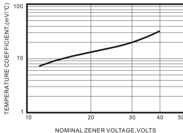
Fig.2 TEMPERATURE COEFFICENTS
