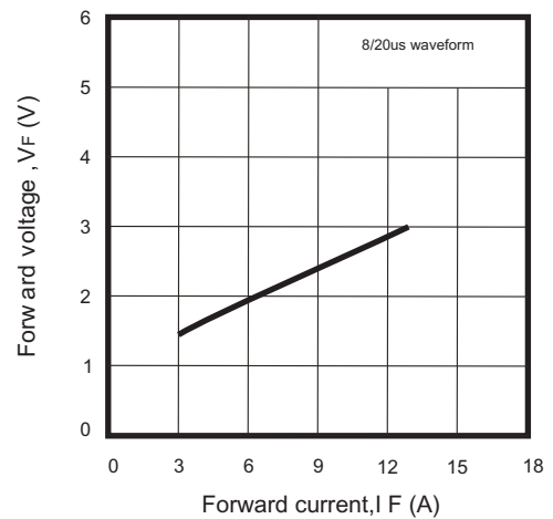
Fig. 4 - Forward volatage vs. forward current
