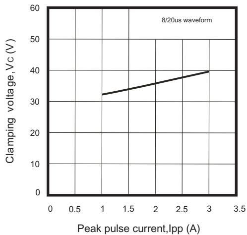
Fig. 3 - Clamping volatage vs. peak pulse current
